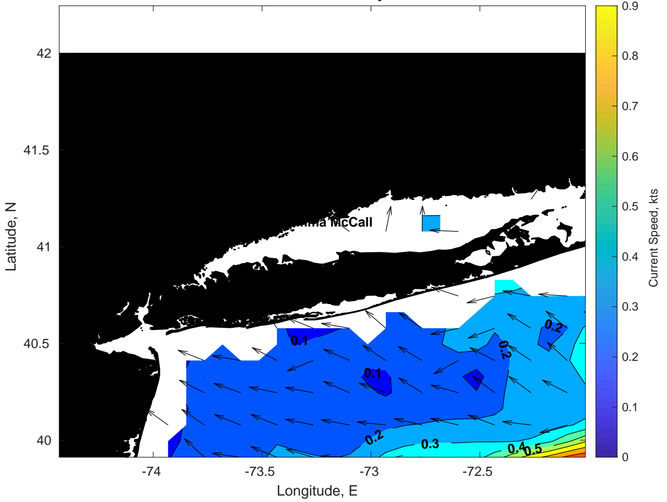
Surface Currents for Emma McCall at 05-May-2024 00:00:00
